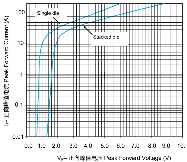
FIGURE 8 峰值正向电压及电流(典型值) Peak Forward Drop vs Peak Forward Current (Typical Values)
