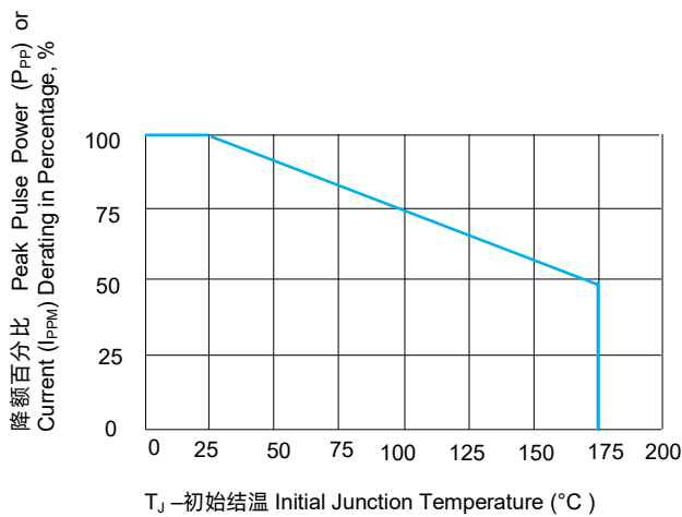
FIGURE 3 峰值脉冲功率降额曲线 Peak Pulse Power Derating Curve
