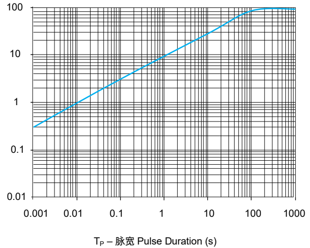
FIGURE 6 典型瞬态热阻 Typical Transient Thermal Impedance
