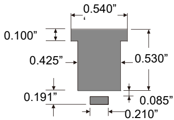
安装布局 Mounting Pad Layout (Inch)
