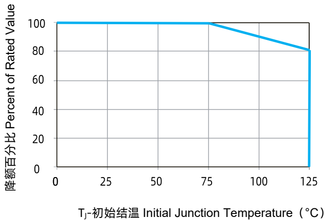
FIGURE 1 峰值功率降额 Peak Power Derating
