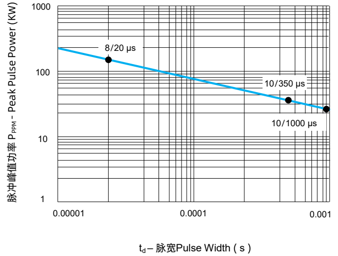
FIGURE 2 典型峰值脉冲功率额定曲线 Typical Peak Pulse Power Rating Curve
