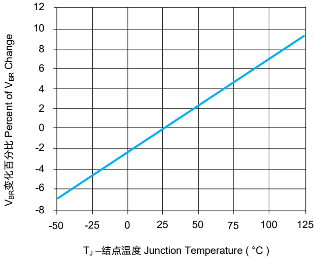
FIGURE 3 典型 V_{BR} 随结温变化曲线 Typical V_{BR} vs T_J Junction Temperature
