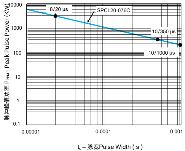
FIGURE 4 峰值脉冲功率额定曲线 Peak Pulse Power Rating Curve
