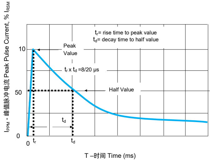
FIGURE 2 脉冲波形 Pulse Waveform
