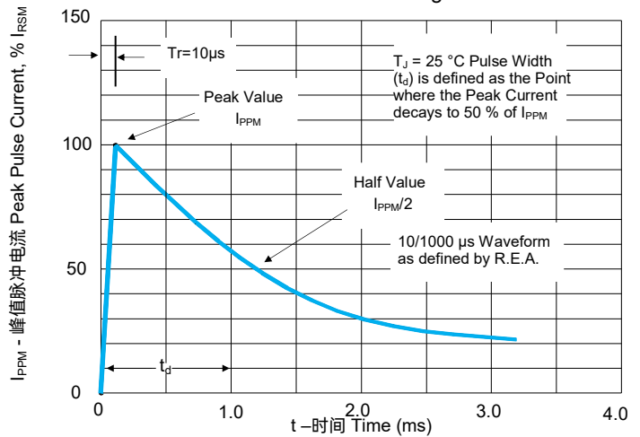
FIGURE 4 脉冲波形 Pulse Waveform
