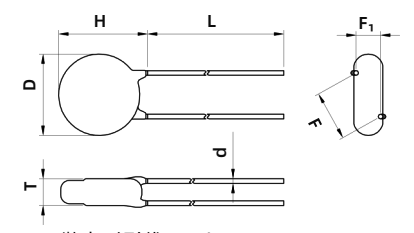
微直型引线 Little Straight Lead
