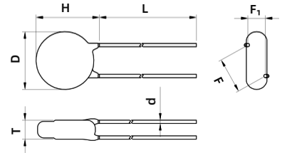
微直型引线 Little Straight Lead
