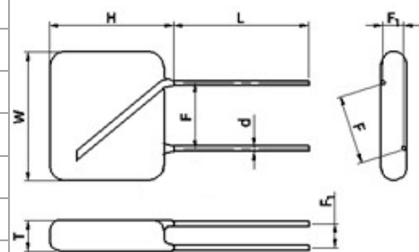
全引线型A All Lead Wire A
