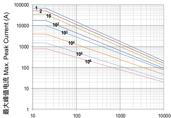
脉冲持续时间 Impulse Duration ( \mu s) SFV53D820K to SFV53D122K
