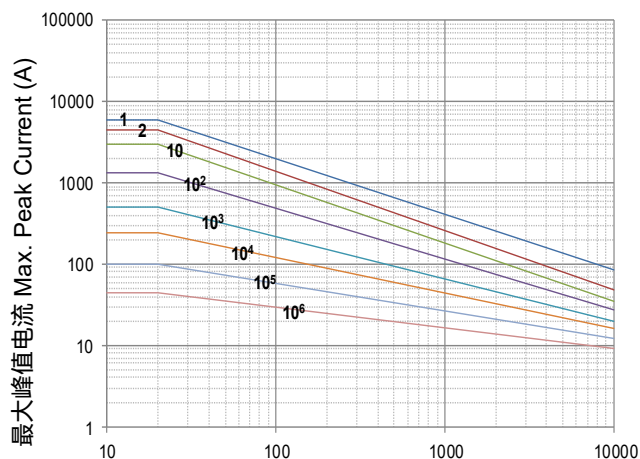
脉冲持续时间 Impulse Duration ( \mu s) SFV25D220K to SFV25D680K
