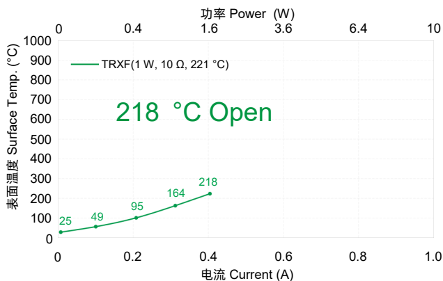
TRXF表面温度曲线(仅供参考) Surface Temp. Curve of TRXF (For reference only)
