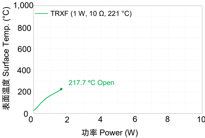
TRXF表面温度曲线 Surface Temp. Curve of TRXF
