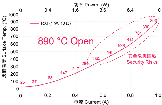
RXF表面温度曲线(仅供参考) Surface Temp. Curve of RXF (For reference only)
